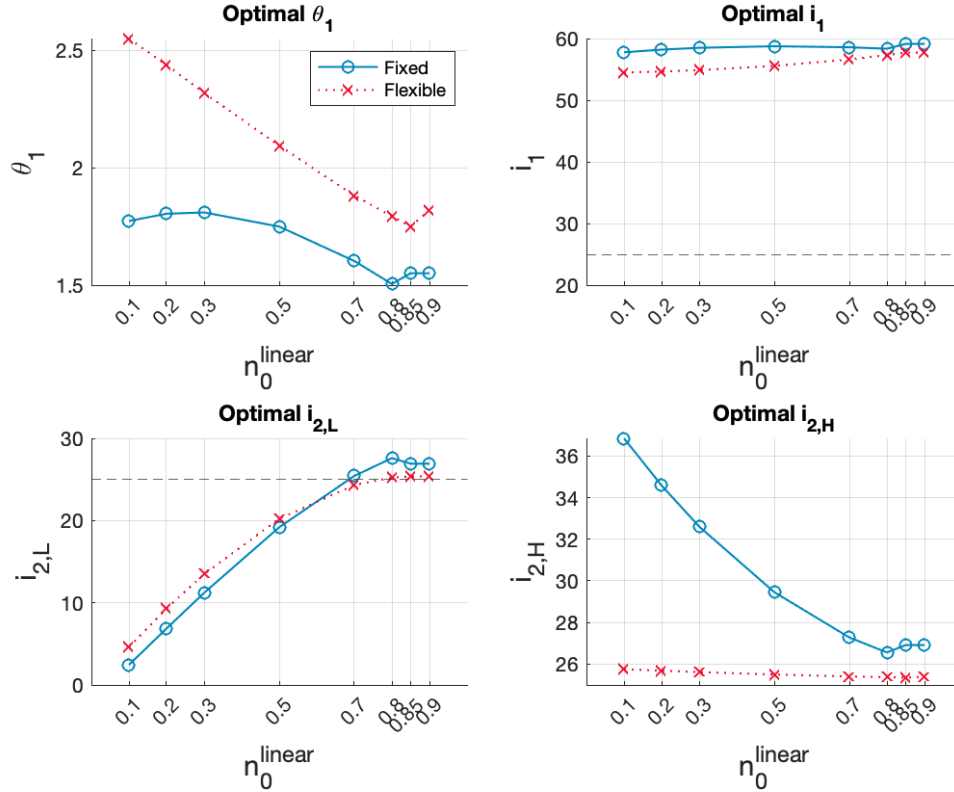
Figure 5: Supplemental Result 2 – change in n_0^{linear}
